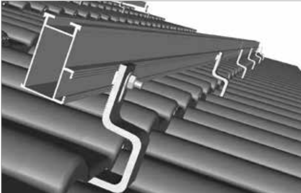
Tiled roof installation with roof hooks
